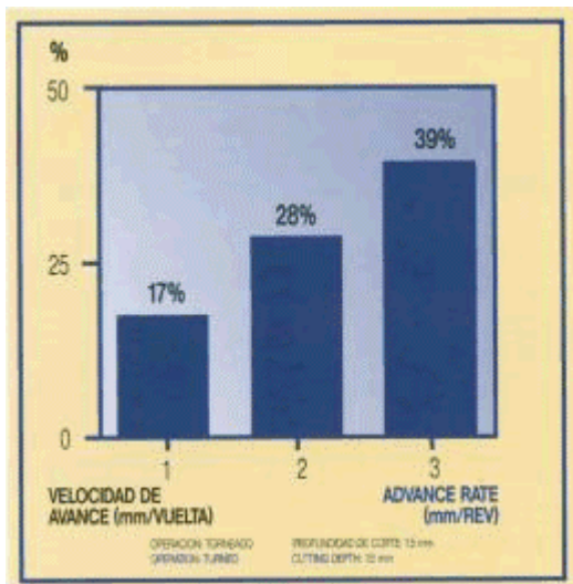
CUTTING RATE INCREASE OF ROLDAMAX OVER THE STANDARD 304 DEPENDING ON THE ADVANCE RATE
