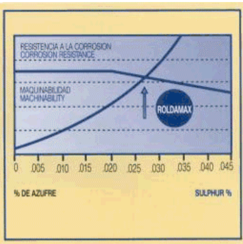
MACHINABILITY AND CORROSION RESISTANCE DEPENDING ON SULPHUR CONTENT
